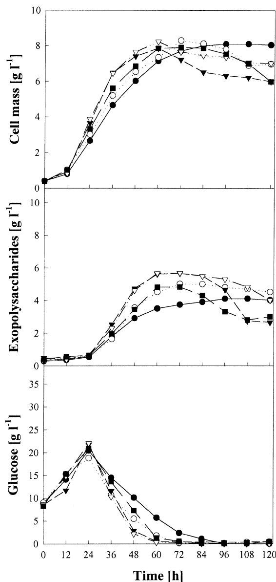
Fig. 6. Effects of DOC and its control method on the cell growth and EPS production in batch culture of A. blazei (●: No DOC control, ○: 10%, ▼: 20%, ▽: 40%, ■: 20% by manipulating pure oxygen supply).
